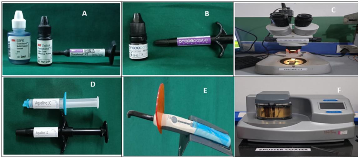
Figure 1: A): ScotchBond Etchant 32% Orthophosphoric acid, Transbond XT Primer, Transbond X Adhesive; B) Bracepaste Primer, Bracepaste Adhesive; C): StereoMicroscope; D) : Aqualine LC Etchant gel, Aqualine LC Bondingpaste; E): 3M S10 ELIPAR Light Curing Unit (3M Unitek); F) Sputter coater Quorum Q150T ES (UK) for gold sputtering of samples. Acrylic jigs with color tags were used for easy identification and shear bond strength measurement, exposing only the tooth crown and paralleling labial force.
